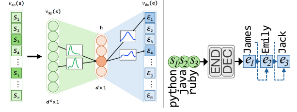
Figure 4: Multilabel vs. seq-to-seq team recommendation. between experts from the easy popular experts to the hard non-popular ones to overcome models' popularity bias (Figure 5).
